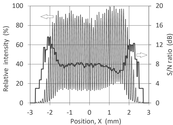
Beam Parallelism
