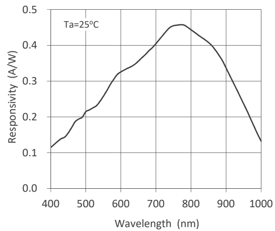
Spectral Responsivity
