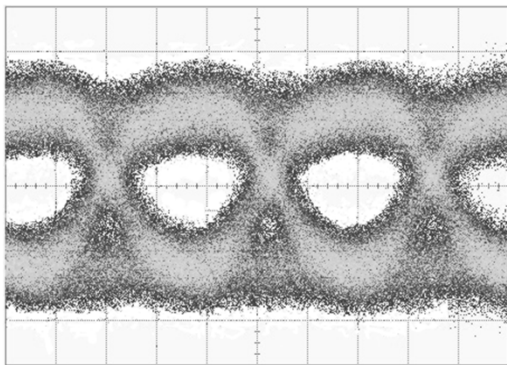
Eye Diagram
